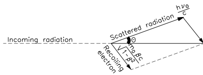
FIGURE 6.3.1. Compton scattering
